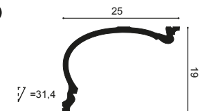
C343 HERITAGE A 200 x 19 x 25 cm Purotouch ®
